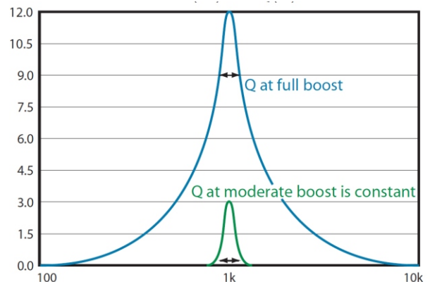
Figure 4. Constant-Q Graphic
